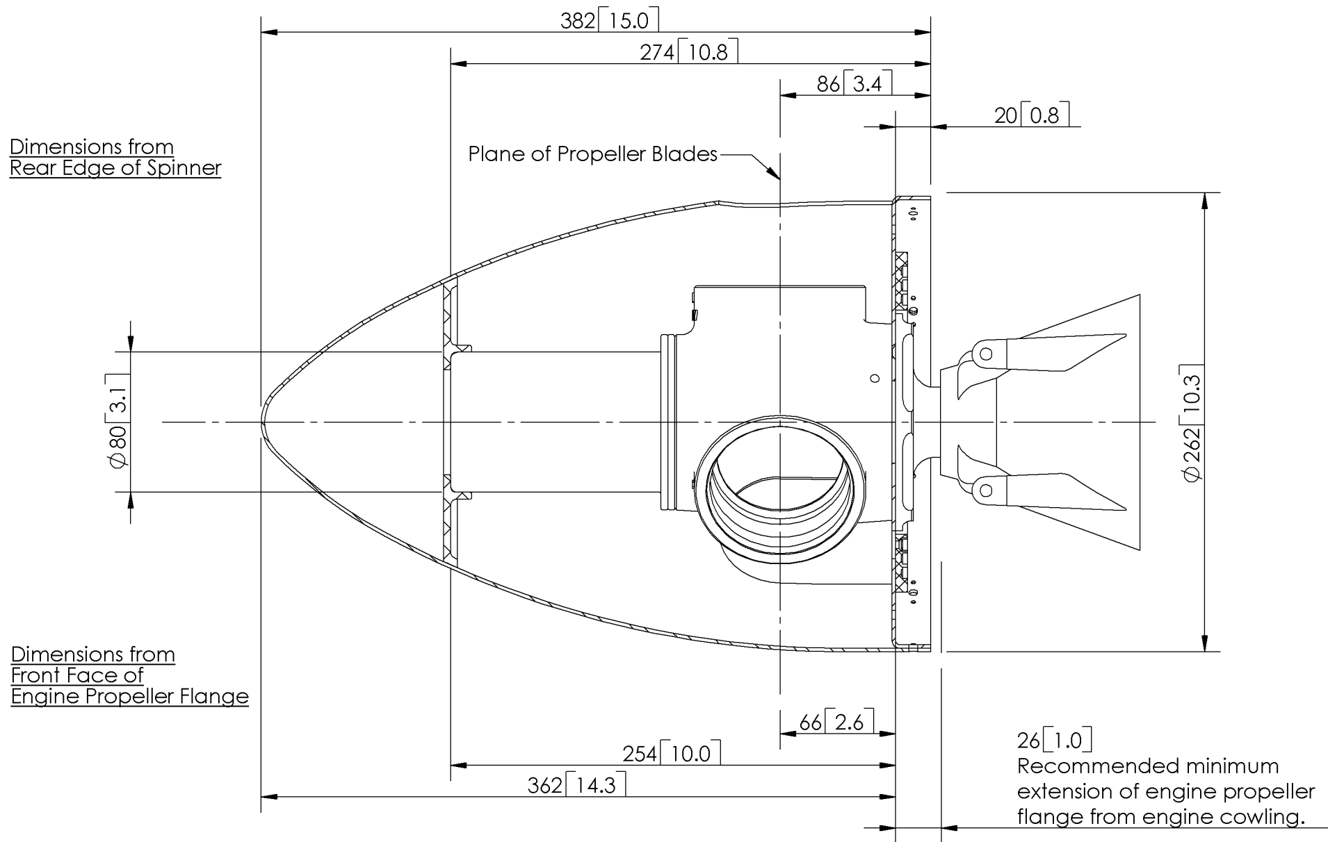
Principal Dimensions of AP332 Propeller with \phi 262\text{mm} (10.3in) Spinner (Example shown mounted on Rotax engine) Primary dimensions in millimeters [secondary dimensions in inches]
